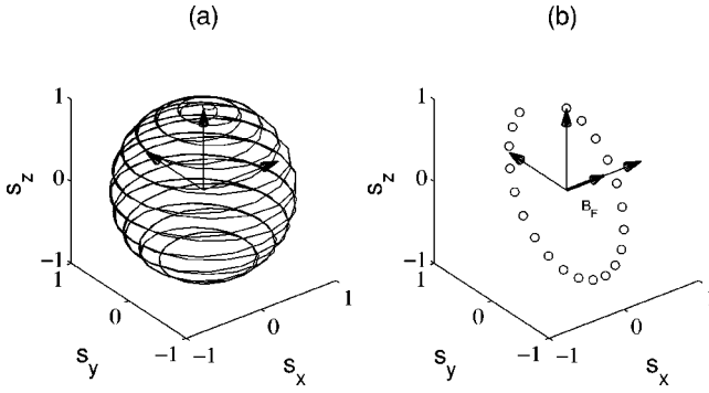
FIG. 3. Analyzing the system in a Floquet basis allows one to replace the (a) complicated continuous dynamics associated with a time dependent Hamiltonian with a (b) simple discrete dynamics associated with Larmor precession about a fictitious static magnetic field, \mathbf{B}_F . The two pictures agree exactly at these discrete times corresponding to integer multiples of the drive period.
