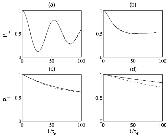
FIG. 4. Comparison of numerical simulations (dotted line) to analytic expressions (solid line). Each graph plots the probability P_L to be in the left well vs time t/\tau_d , for the parameters A_x=0.1 , A_z=1.1 , and \omega_d=1 . There is excellent agreement for (a) underdamped ( \sigma=0.20 , T_2=50\tau_d ), (b) critically damped ( \sigma=0.68 , T_2=4.28\tau_d ), and (c) overdamped ( \sigma=1.41 , T_2=1\tau_d ) cases. The model breaks down [(d) ( \sigma=2.5 , T_2=0.32\tau_d )] when T_2 < \tau_d .
