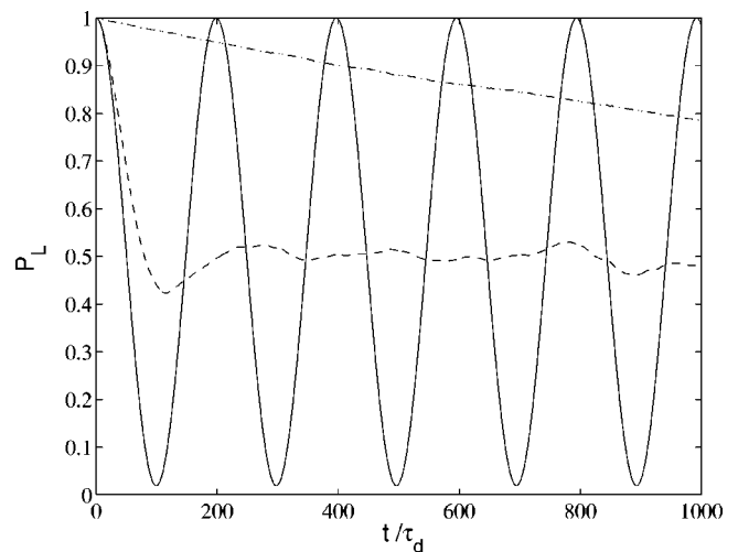
FIG. 1. The probability to be in the left well, P_L , vs time t/\tau_d . For the central cosinusoidal curve (solid line) \sigma=0 , where \sigma is the root mean variance of the probability distribution which governs the discrete random variable, we have coherent oscillations between the |L\rangle and |R\rangle states at a modified tunneling rate corresponding to the quasienergy splitting. In the central rapidly decaying curve (dashed line), \sigma=0.25 , stochastic \delta -function kicks rapidly destroy coherent oscillations. In the upper, slowly decaying curve (dash-dotted line), \sigma=2.5 , the coherent suppression of tunneling has been partially restored by the increased noise strength. Compare this to Fig. 7b in Ref. [6], and Fig. 2 in Ref. [7].
