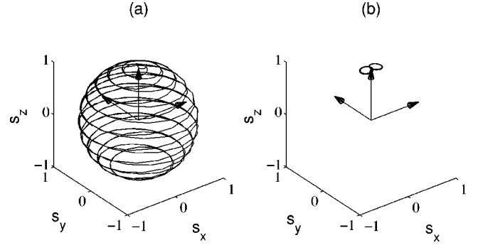
FIG. 2. The representation of coherent suppression of tunneling on the Bloch sphere for a two-level system initially in the |L\rangle state: (a) Trajectories off the condition of coherent suppression of tunneling wind up and down the Bloch sphere. (b) When the condition for coherent suppression of tunneling is met trajectories form closed “loops” near the top ( |L\rangle ) of the Bloch sphere.
